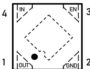
DFN1x1-4
